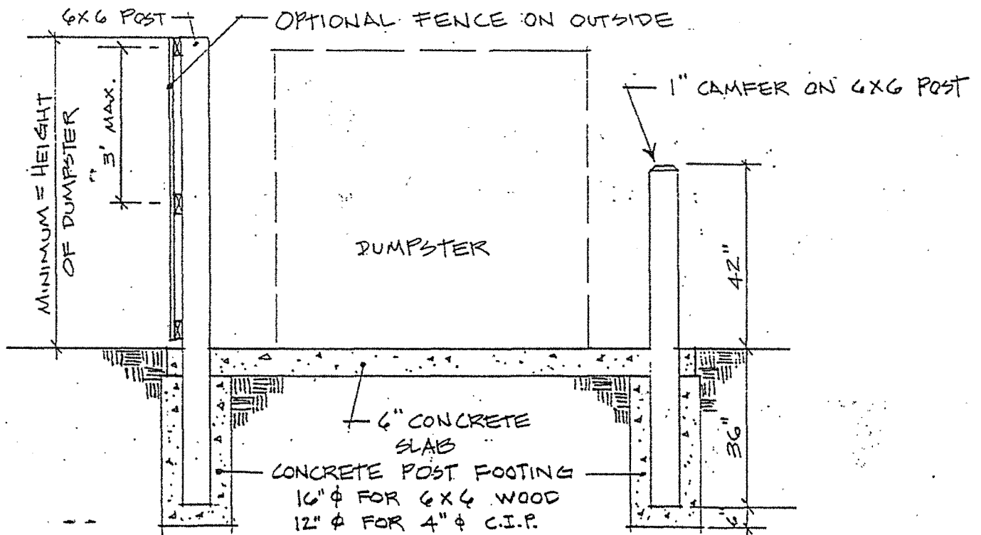
SECTION 3/8"=1'
