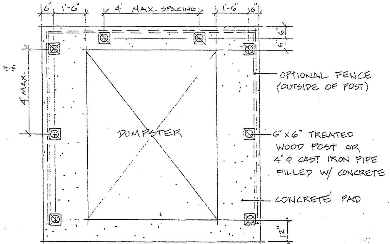
PLAN 3/8"=1'
